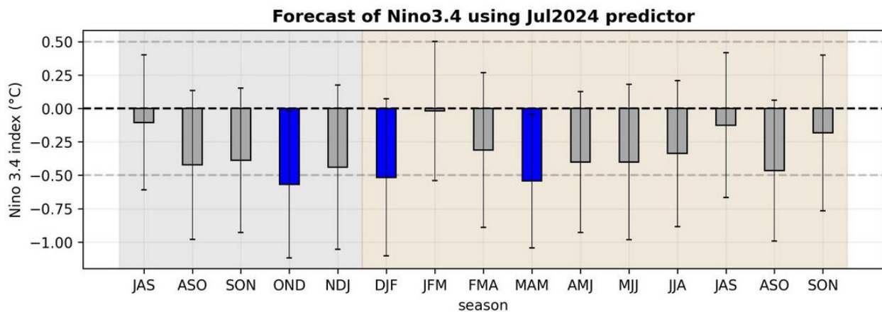
Fig. 4: Median prediction of Nino 3.4 index using May to July, 2024 predictors for the upcoming seasons.
