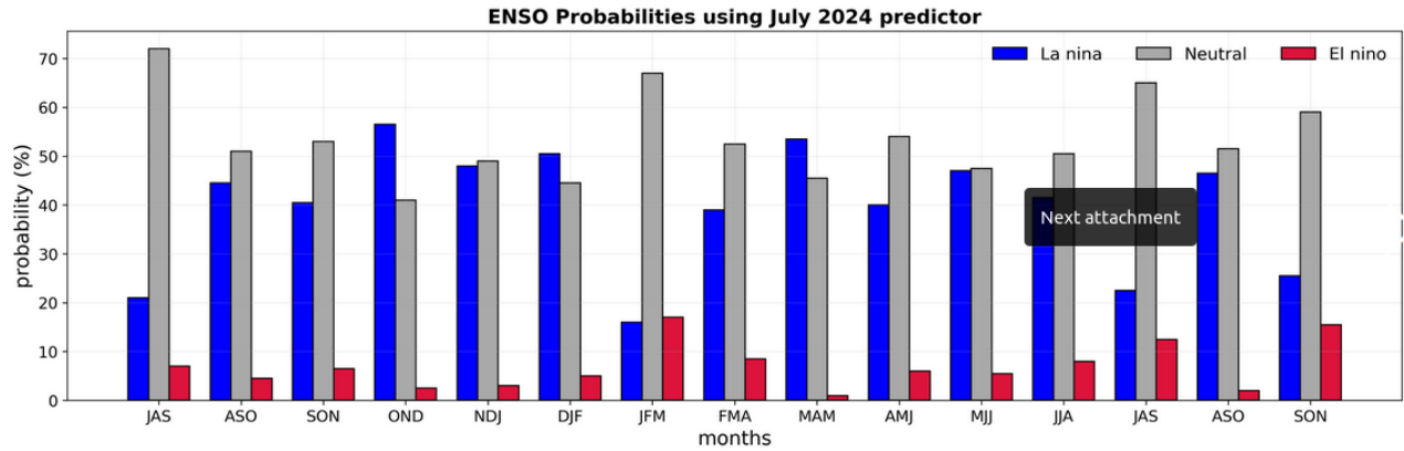
Fig. 5. Forecast of El Nino/La Nina conditions using May to July, 2024 predictors.
