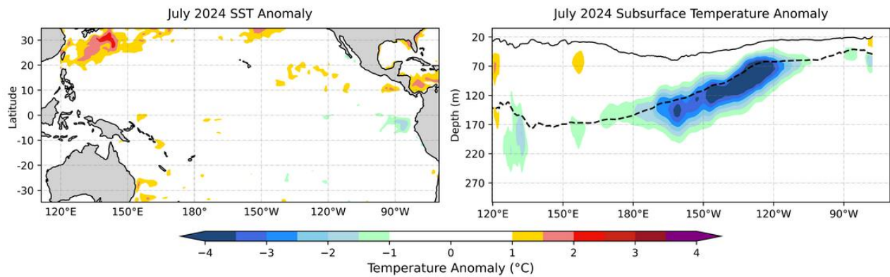
Fig. 3: (Left) Monthly SST anomaly for the tropical Pacific in July 2024. (Right) Subsurface temperature anomaly averaged over 5° S-5° N for July 2024.
