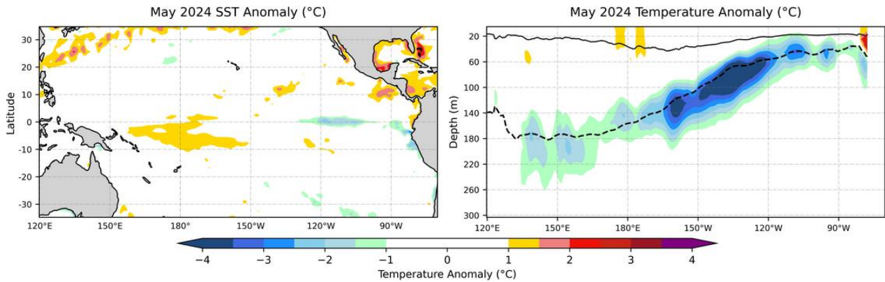
Fig. 3: (Left) Monthly SST anomaly for the tropical Pacific in May 2024. (Right) Subsurface temperature anomaly averaged over 5° S-5° N for May 2024.
