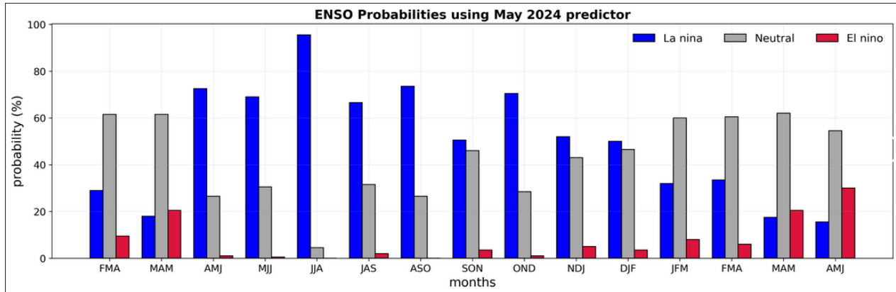
Fig. 5. Forecast of El Nino/La Nina conditions using March 2024-May 2024 predictors.
