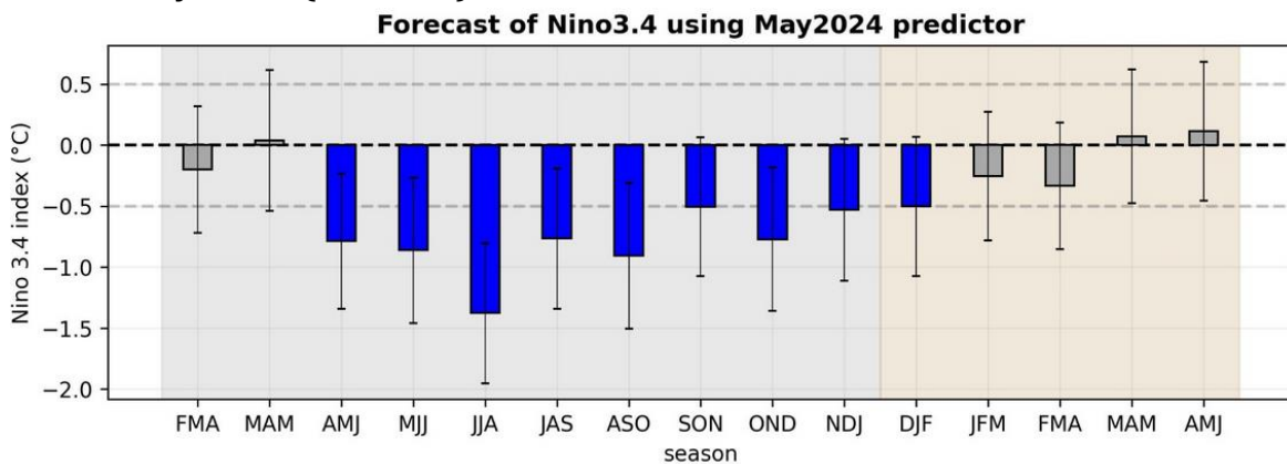
Fig. 4: Median prediction of Nino 3.4 index using March 2024-May 2024 predictors for the upcoming seasons.
