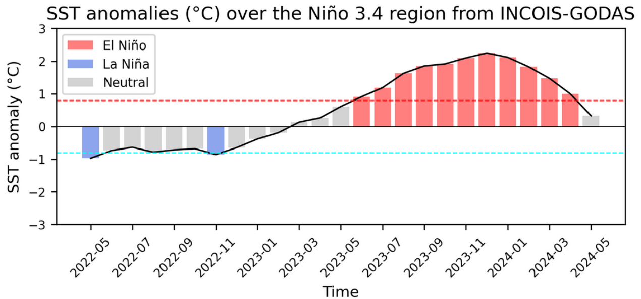
Fig. 1: Evolution of Sea Surface Temperature anomalies (°C) in the Niño 3.4 (5°S-5°N, 170°W-120°W) region in the period May 2022-May 2024. The RED and CYAN horizontal lines represent 0.8°C SST anomaly
