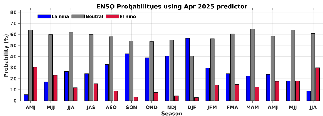
Fig. 5. Forecast of El Nino/La Nina conditions using February 2025-April 2025 predictors.
