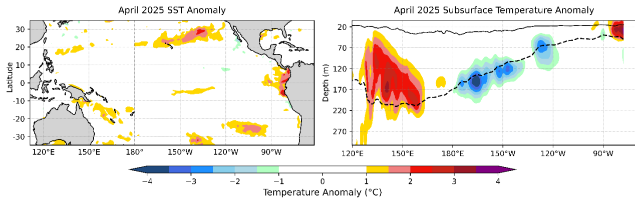
Fig. 3: (Left) Monthly SST anomaly for the tropical Pacific in April 2025. (Right) Subsurface temperature anomaly averaged over 5° S-5° N for April 2025.
