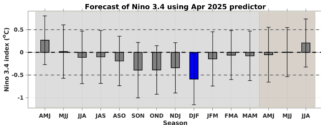
Fig. 4: Median prediction of Nino 3.4 index using February 2025-April 2025 predictors for the upcoming seasons.
